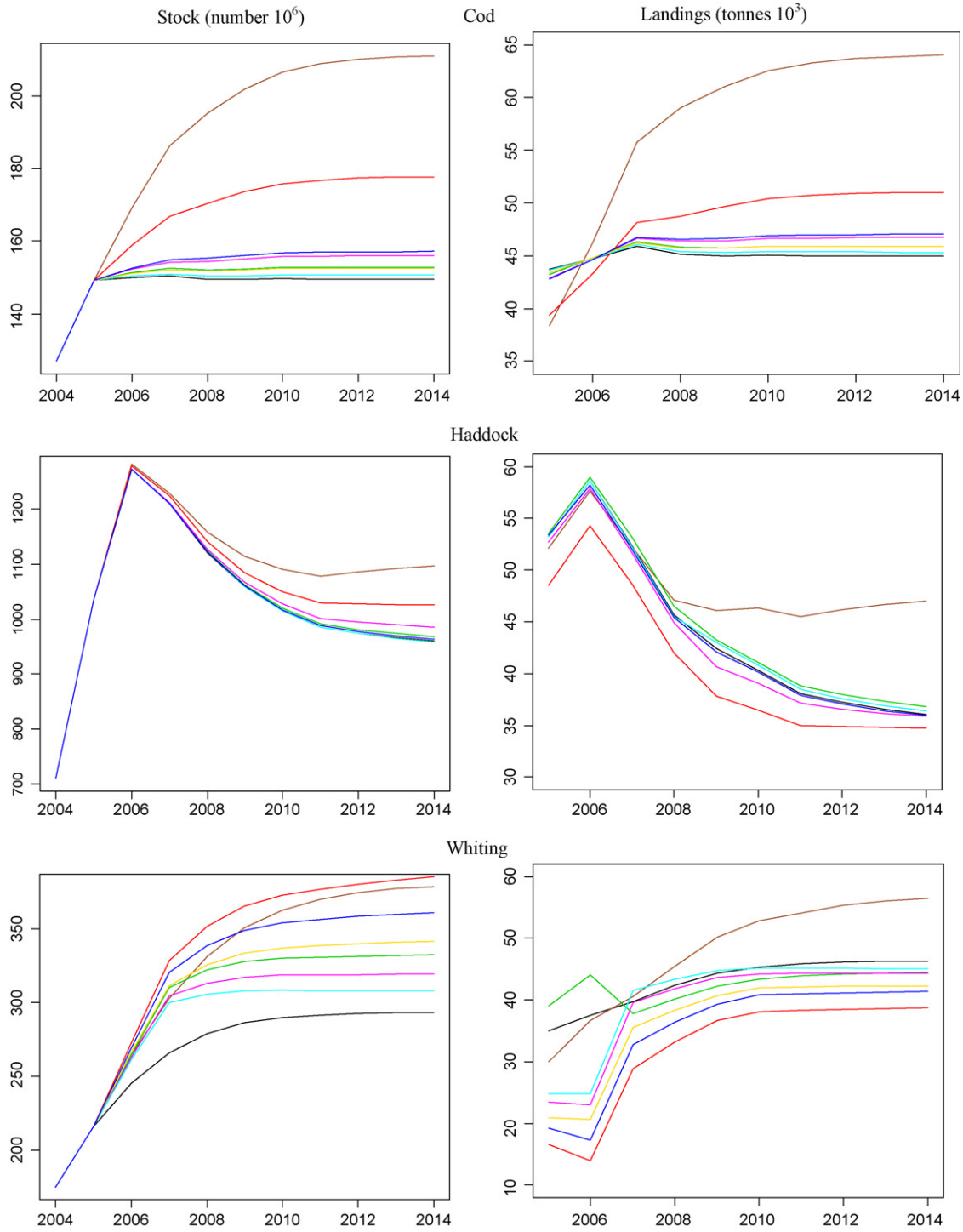
Fig. 2. Model output for forecast stock (number 10^6 ) and landings (weight) of North Sea cod, haddock and whiting comparing the baseline run (black) with the scenarios of no discarding in any fishery (brown), no discarding in Nephrops fisheries (green) and the following trawl designs in Nephrops fisheries: Dyneema SMP (pink), grid and SMC (red), two SMPs (turquoise), Cutaway trawl (yellow) and 100 mm codend (blue). (For interpretation of the references to color in this figure legend, the reader is referred to the web version of the article.)
