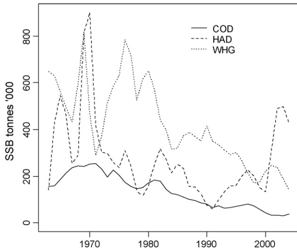
Fig. 1. Output from replicated ICES assessments for North Sea cod, haddock and whiting, illustrating trends in spawning stock biomass.
