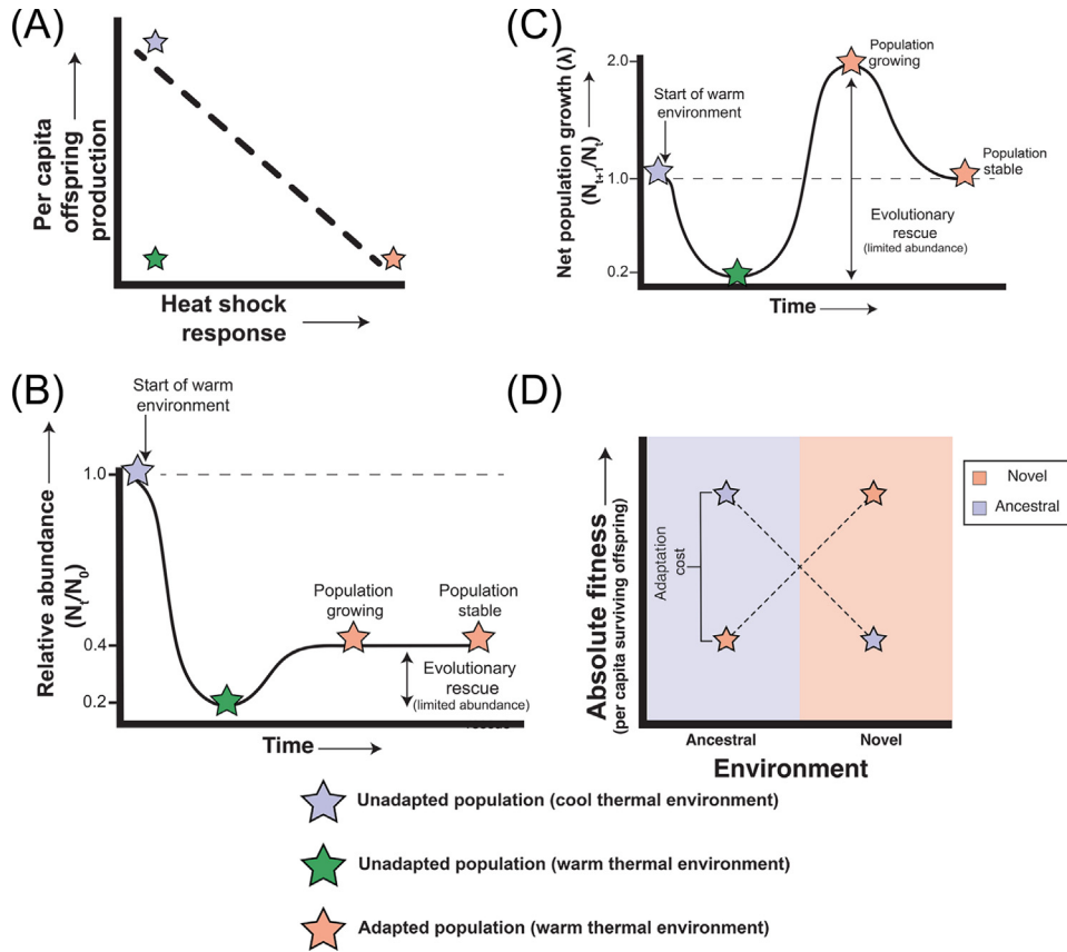
Figure 1. Adaptation with costs because of trade-offs. Colored stars (bottom legend) indicate an unadapted population in cool, ancestral environments (blue); an unadapted population in a warm, novel environment (green); and an adapted population in a warm, novel environment (pink). (A) The trade-off relationship between per capita offspring production and heat-shock response. (B) Changes in population abundance [relative to the starting (blue) generation]. Evolutionary rescue recovers population abundance to a fraction of the ancestral generation level. The relative abundance of the adapted (pink) population here reaches a plateau after recovery. (C) The observed net population growth ( \lambda ; N_{t+1}/N_t ) for three sequential generations adapting to temperature changes where each generation has the same generation time. The net population growth of the warm (pink) generation is higher than the cool (blue) population because \lambda is estimated on the basis of abundance measures of the preceding (green) generation, not the initial (blue) generation. (D) The test of adaptation costs. Costs of adaptation are inferred if the fitness of the adapted (pink) population declines when experiencing ancestral foreign (blue) environments.
