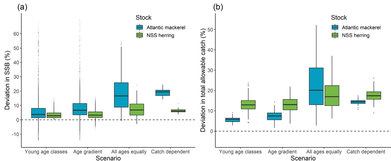
Figure 3. Boxplots of percentage deviations in annual SSB (a) and total allowed catch (b) for NEA mackerel (blue) and NSS herring (green) between scenarios with increased mortality and baseline run without increased mortality. Deviations in SSB were summarized over the entire time series and all bootstrap runs, whereas deviations in TAC are shown for the year following the last assessment year (here 2018). TAC forecasts are based on the Fmsy-rule ( F = 0.23 and F = 0.156 , respectively, for mackerel and herring) for each stock. Two of the scenarios were age-dependent (only the youngest age classes or a decreasing effect with age), while two were age-independent (i.e. all ages affected equally), including on where the effect strength is affected by total annual catches. The boxplots show median (solid black line), first and third quartiles (lower and upper bounds of the boxes), 1.5 times the interquartile range (whiskers), and the outliers outside of this range (dots), over all bootstrapped runs for each scenario.
