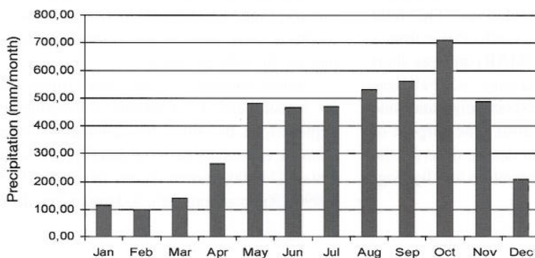
Fig. 2. Monthly precipitation (mm/month) in the catchment basin of Golfo Dulce (Herrera 1985).
