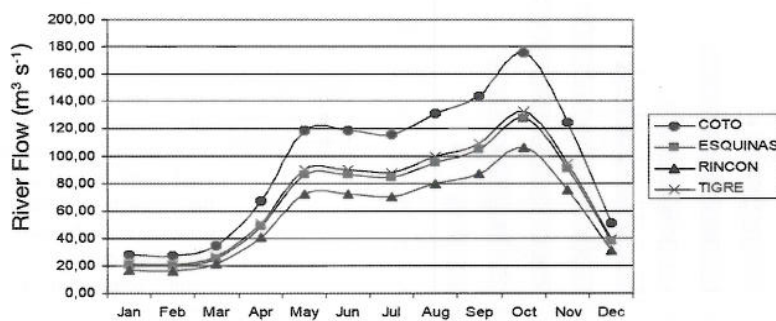
Fig. 3. Estimated freshwater discharge from the four main rivers (Coto, Esquinas, Rincón and Tigre) entering Golfo Dulce (Herrera 1985).
