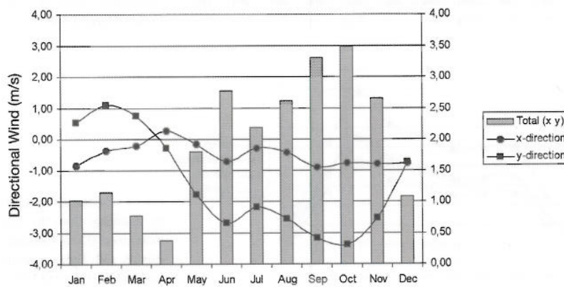
Fig. 5. The lines show the 180° rotated x, y-vector components ( m s^{-1} ) of the wind used in the model. Bars present total surface wind ( m s^{-1} ) calculated as the vector product of the x and y components (Oort 1983).
