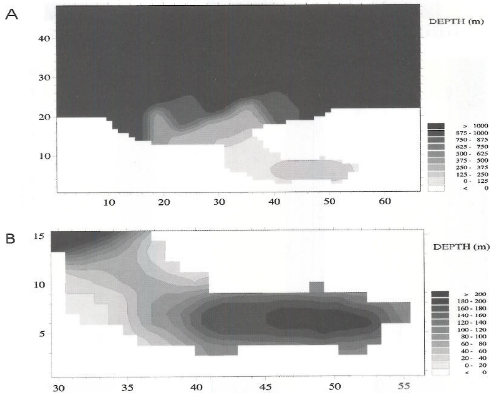
Fig. 11. The bottom topography of the total model area (A) and the bottom topography of Golfo Dulce (B). The scales to the right show the depths corresponding to each contour.
