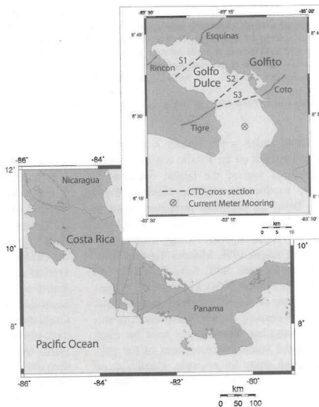
Fig. 1. Sketch of Costa Rica and of Golfo Dulce showing the positions of the CTD-transsects S1-S3, the position of the current meter mooring and the main rivers.
