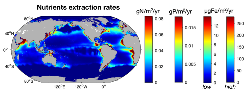
Figure 7. Distribution of the modeled amount of N ( \text{g N m}^{-2} \text{ yr}^{-1} ), P ( \text{g P m}^{-2} \text{ yr}^{-1} ), and Fe ( \mu\text{g Fe m}^{-2} \text{ yr}^{-1} ) extracted from the ocean at the time of the global peak catch. The two color bars for Fe represent the low and high estimates based on the 95 % confidence interval for Fe : C values in fish ( 10\text{--}200 \mu\text{mol Fe (mol C)}^{-1} ).
