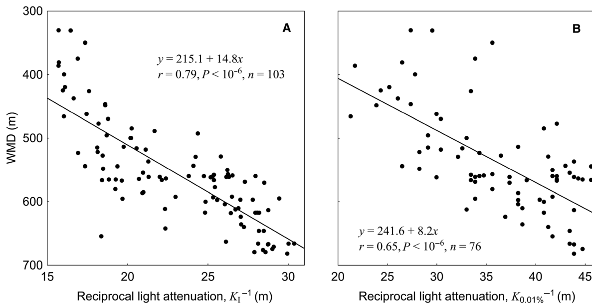
Fig. 3. DSL daytime depth in relation to light penetration. The WMD of the DSL plotted against the reciprocal light attenuation coefficient that is (A) modeled ( K_I ) for the entire water column down to 1000-m depth and (B) estimated ( K_{0.01\%} ) from irradiance measurements conducted in the upper water masses down to 0.01% light depth.
